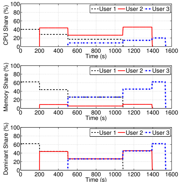
Fig. 4. CPU, memory, and global dominant share for three users on a 100-server system with 52.75 CPU units and 51.32 memory units in total.
