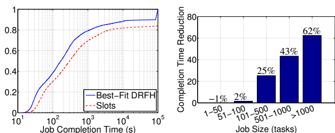
(a) CDF of job completion times. (b) Job completion time reduction.
