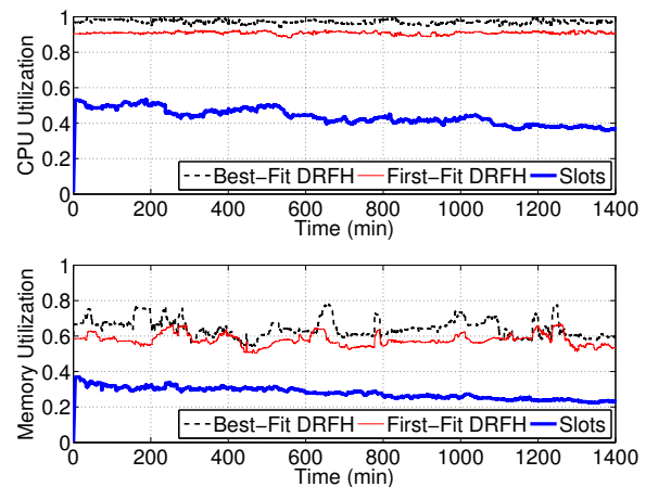
Fig. 5. Time series of CPU and memory utilization.
