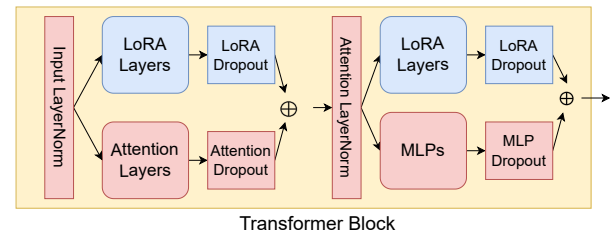
Fig. 2: The structure of a typical transformer block (with LoRA fine-tuning method).
