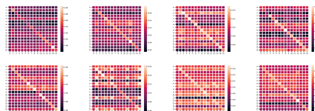
Fig. 21: The similarity of features between the inputs and outputs of the first transformer layer in OPT.
