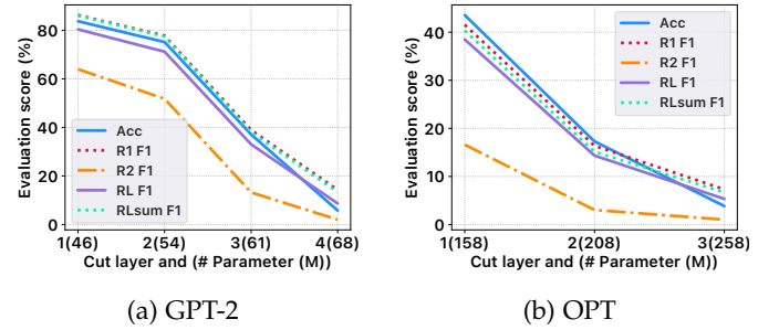
Fig. 3: The attacking results of UnSplit over GPT-2 and OPT with placing different number of transformer layers on the clients, in the first iteration.
