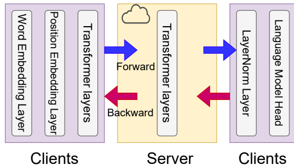
Fig. 1: The deployment of language model across the clients and the server in split learning.
