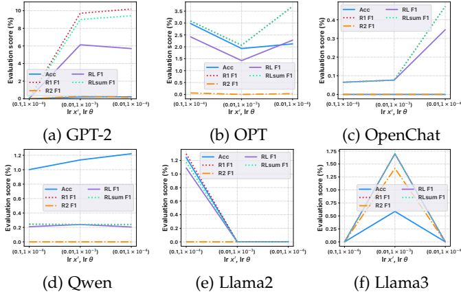
Fig. 6: The attacking results over different models with placing the first transformer layer on the clients, in the second iteration, setting different attacking hyper parameters.
