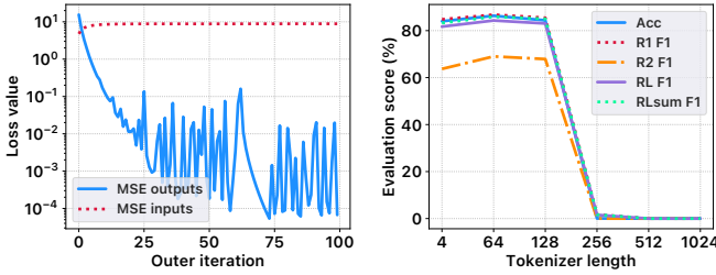
Fig. 14: The change in MSEs during the attack, in the experiments in Table 2 over GPT-2. Fig. 15: Repeat the experiments of the second iteration in Table 2 over GPT-2, by using different tokenizer lengths.
