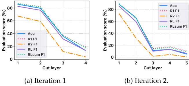
Fig. 7: The attacking results over GPT-2 with placing different number of transformer layers on the clients, in the first and second iteration when dropout layers are disabled.
