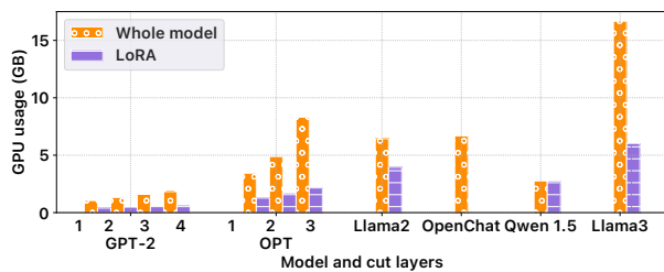
Fig. 22: The GPU memories needed on each clients when training language models with split learning. We place several transformer layers on the clients. The numbers in the x-axis represent the number of layers placed on the clients.
