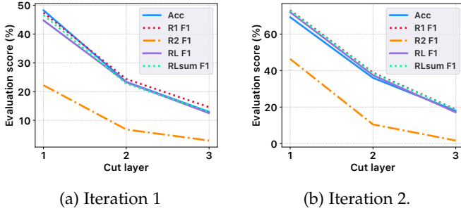
Fig. 8: The attacking results over OPT with placing different number of transformer layers on the clients, in the first and second iteration when dropout layers are disabled.
