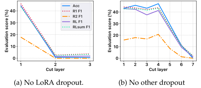
Fig. 9: The attacking results of UnSplit over GPT-2 with placing different number of transformer layers on the clients, in the second iteration and fine-tune with LoRA method. The LoRA dropout layers are disabled and the other dropout layers are disabled respectively in two cases.
