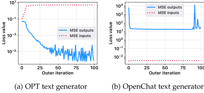
Fig. 13: The change in MSE between outputs of the guessed client model and the intermediate features, and between private embedding features and reconstructed embedding during the attack, in the experiments in Table 4.
