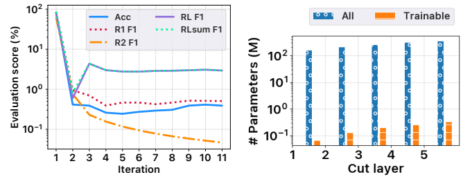
Fig. 4: The attacking results Fig. 5: Parameters and trainable parameters when fine-tuning OPT with LoRA and layer on the clients, during placing different layers on clients.
